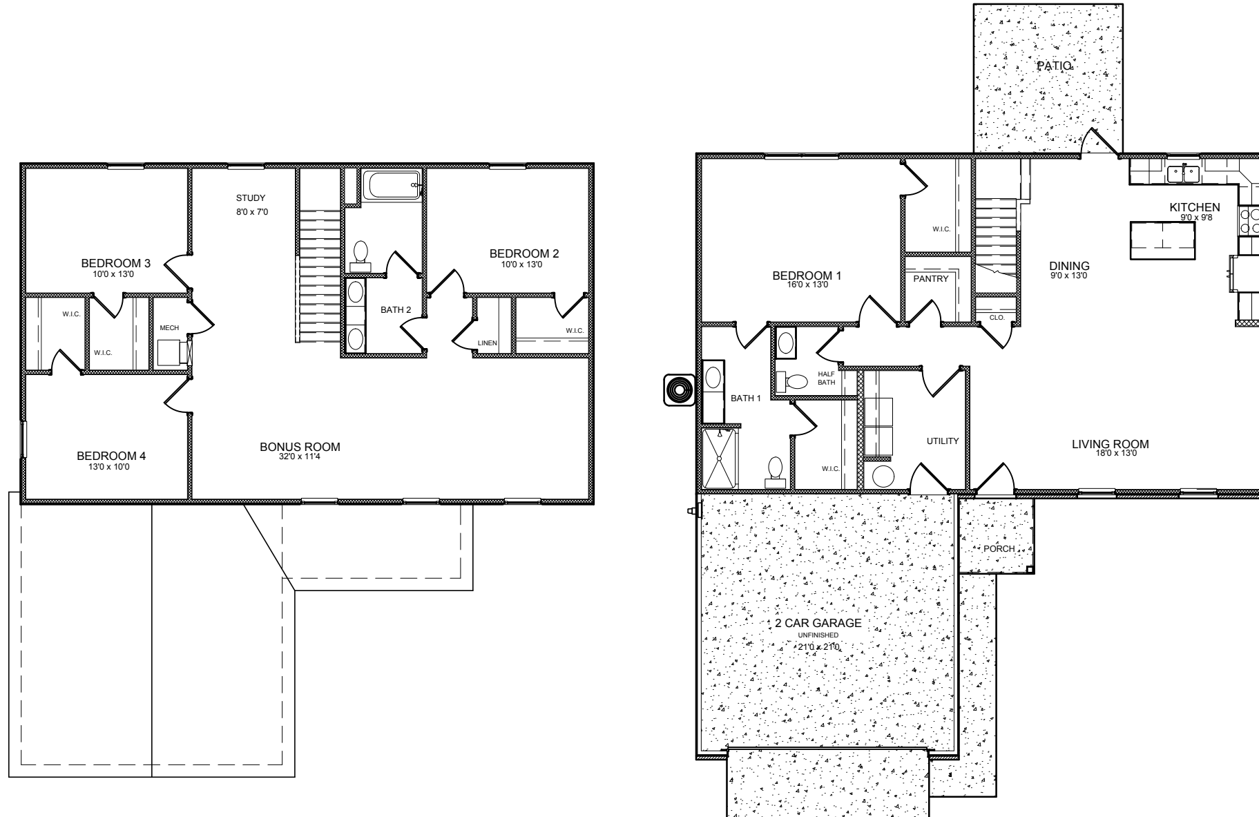
GARAGE OPTION
