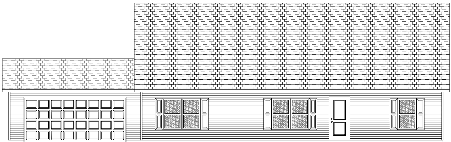
FRONT ELEVATION W/ GARAGE
