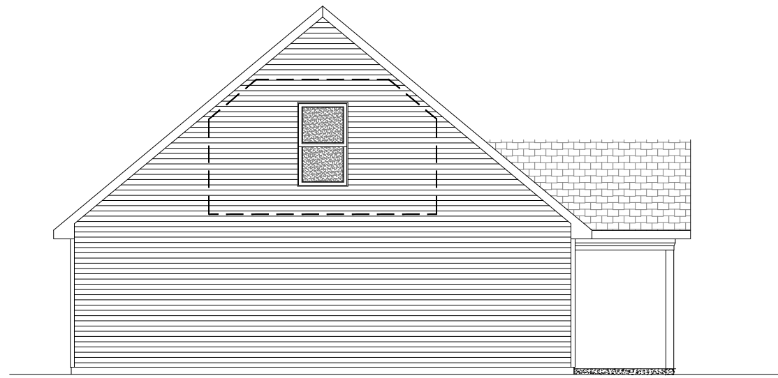
SIDE ELEVATION W/ GABLED ROOF
