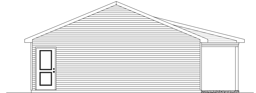
SIDE ELEVATION W/ SHED ROOF
