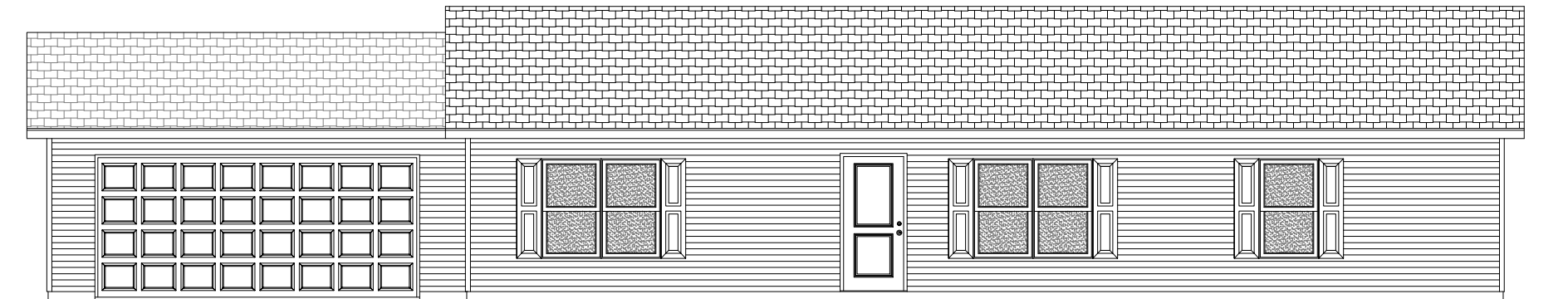
FRONT ELEVATION W/GARAGE
