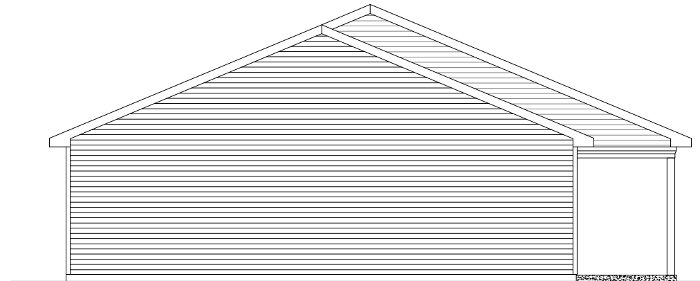
SIDE ELEVATION W/ SHED ROOF
