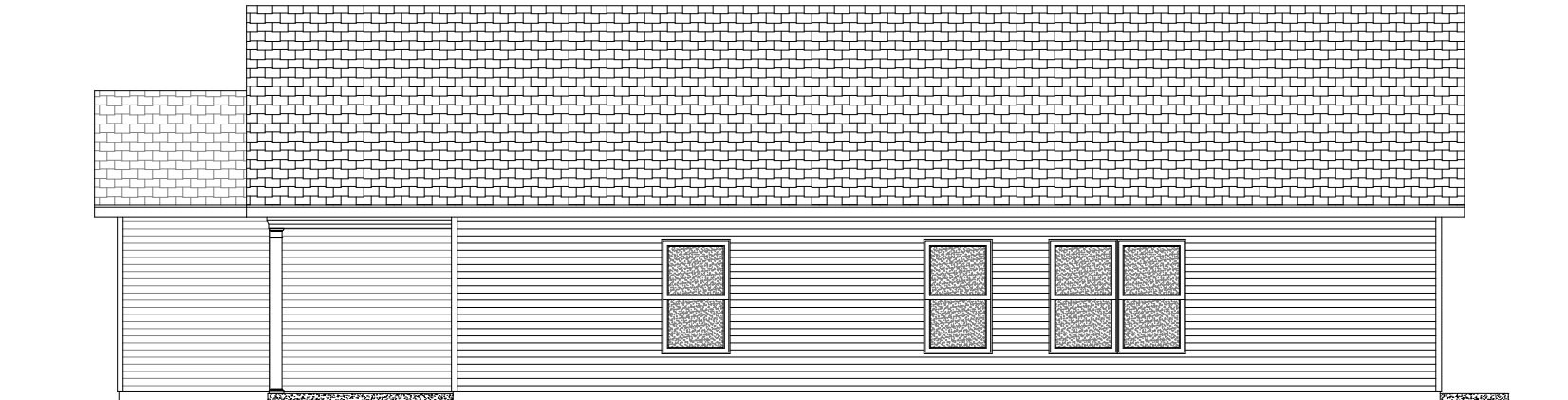
SIDE ELEVATION
