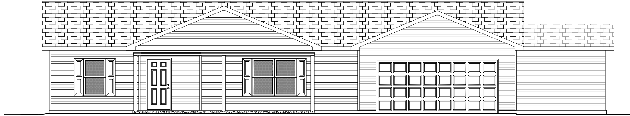
FRONT ELEVATION W/ GARAGE & 24' PORCH
