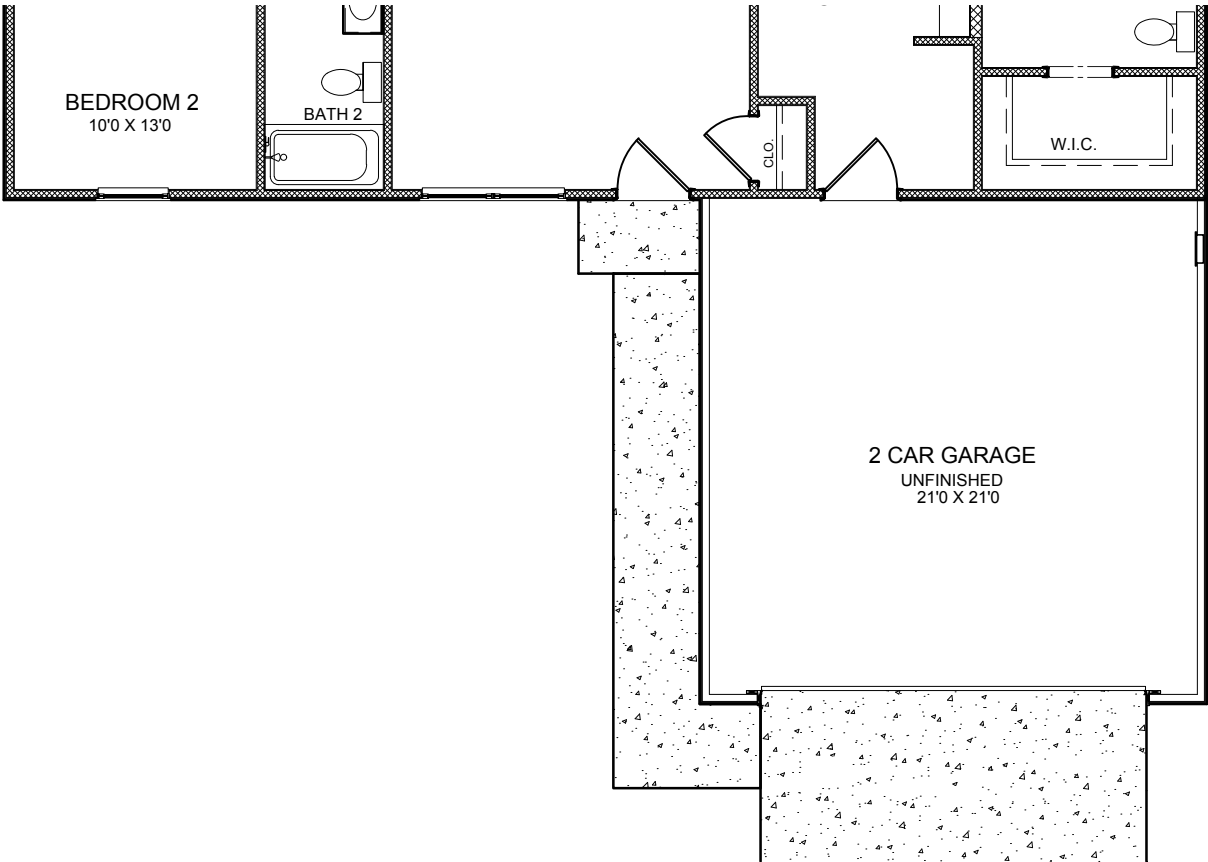
GARAGE OPTION w/ CONCRETE STOOP
