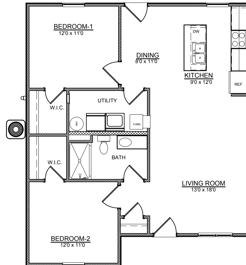
MAIN LEVEL PLAN - 1,013 SF
