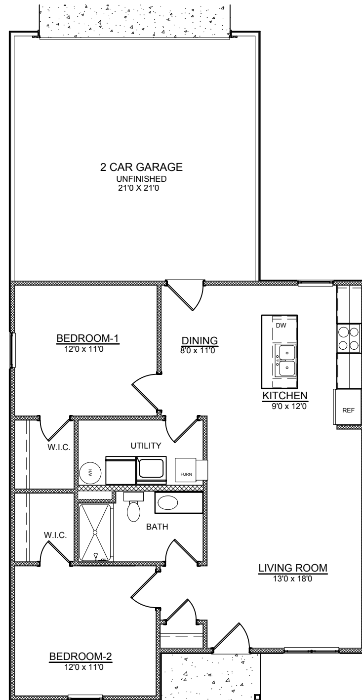
GARAGE OPTION PLAN W/ PORCH
