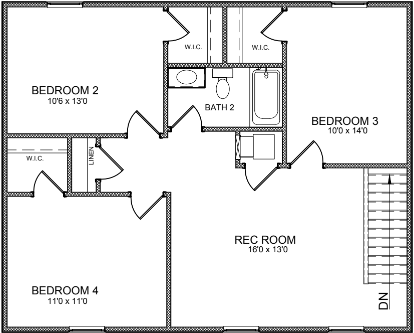
UPPER LEVEL PLAN - 929 SF
