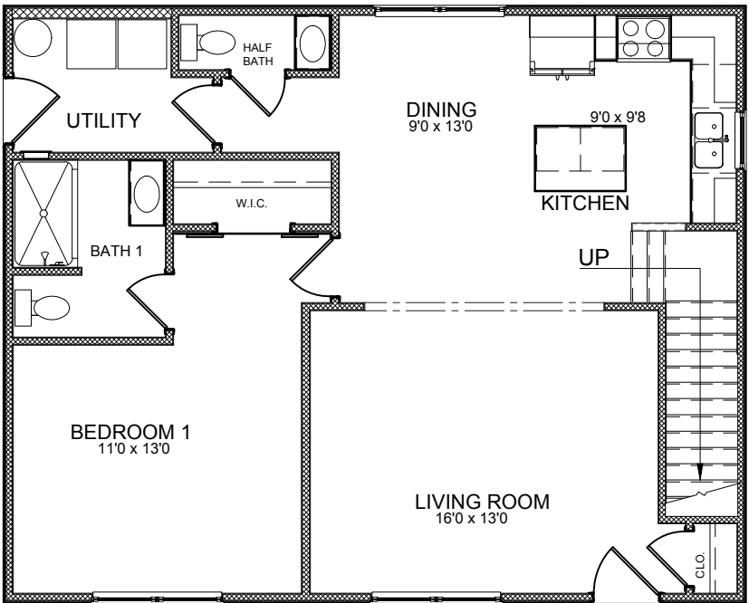
MAIN LEVEL PLAN - 929 SF
