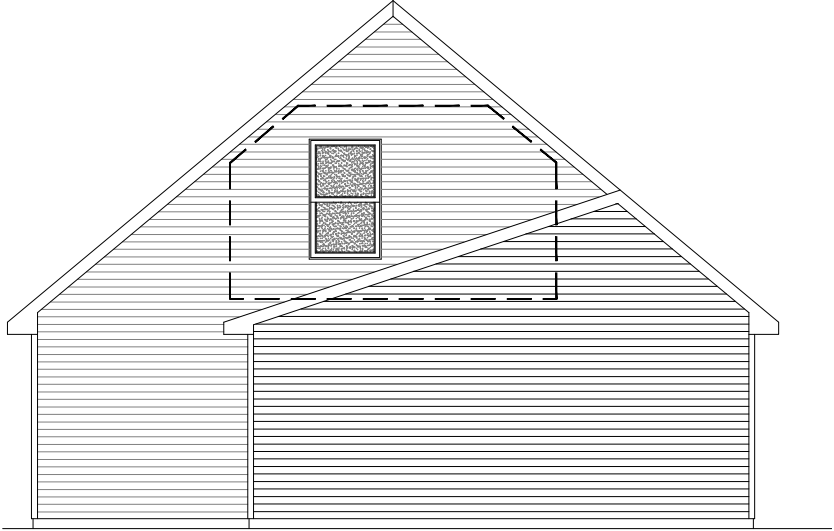
SIDE ELEVATION W/ GARAGE PLAN 'B'; PLAN 'C' SIMILAR
