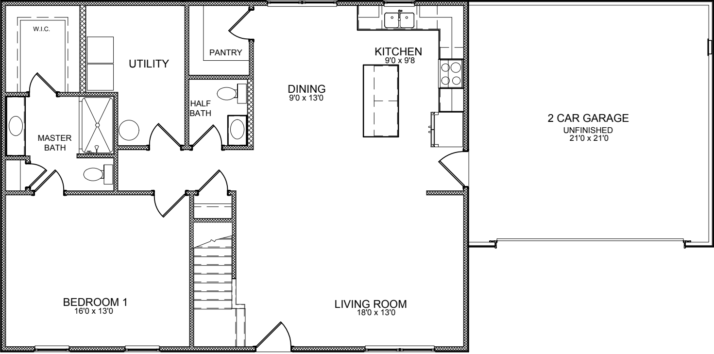
OPTIONAL FLOOR PLAN 'B' W/ GARAGE
