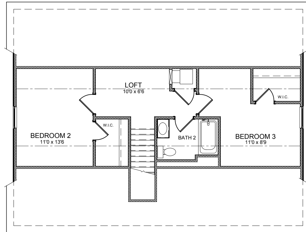
UPPER LEVEL PLAN - 584 SF
