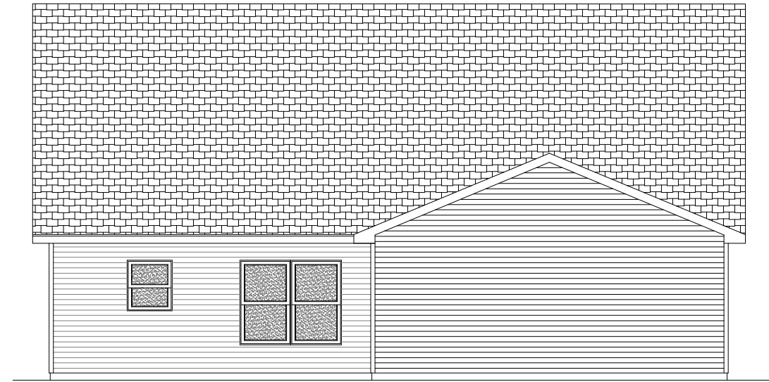
REAR ELEVATION W/ GARAGE
