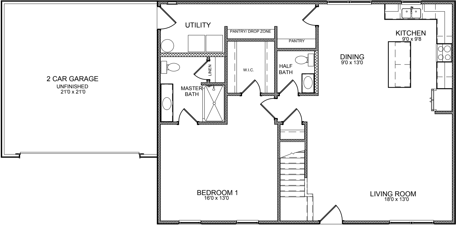
OPTIONAL FLOOR PLAN 'C' W/ GARAGE
