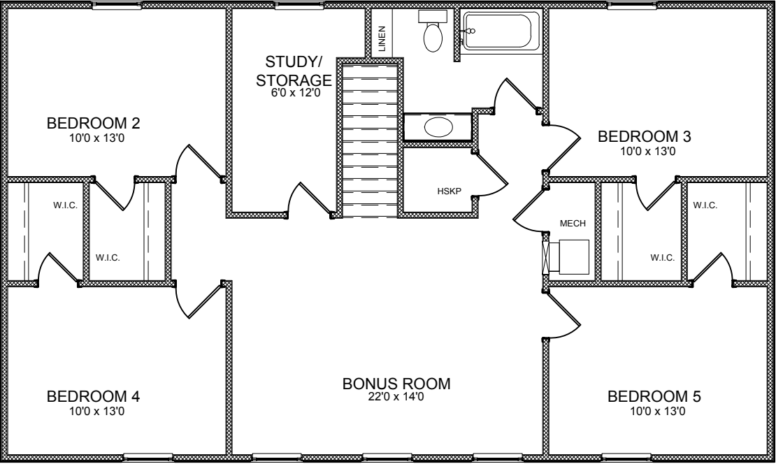
UPPER LEVEL - 1,257 SF
