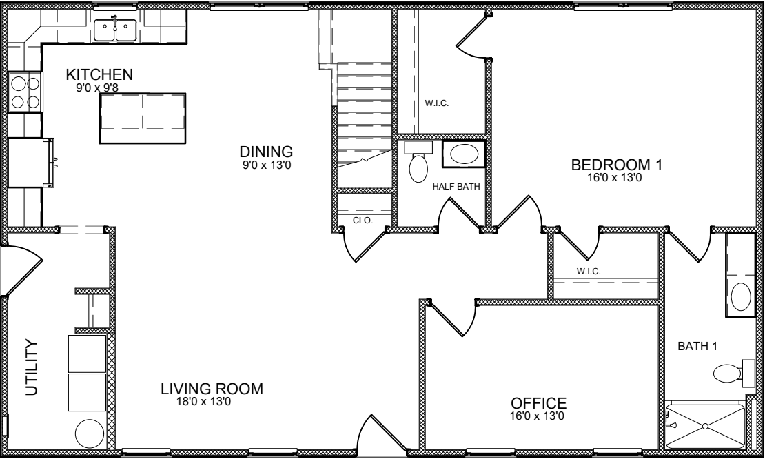
MAIN LEVEL PLAN - 1,257 SF
