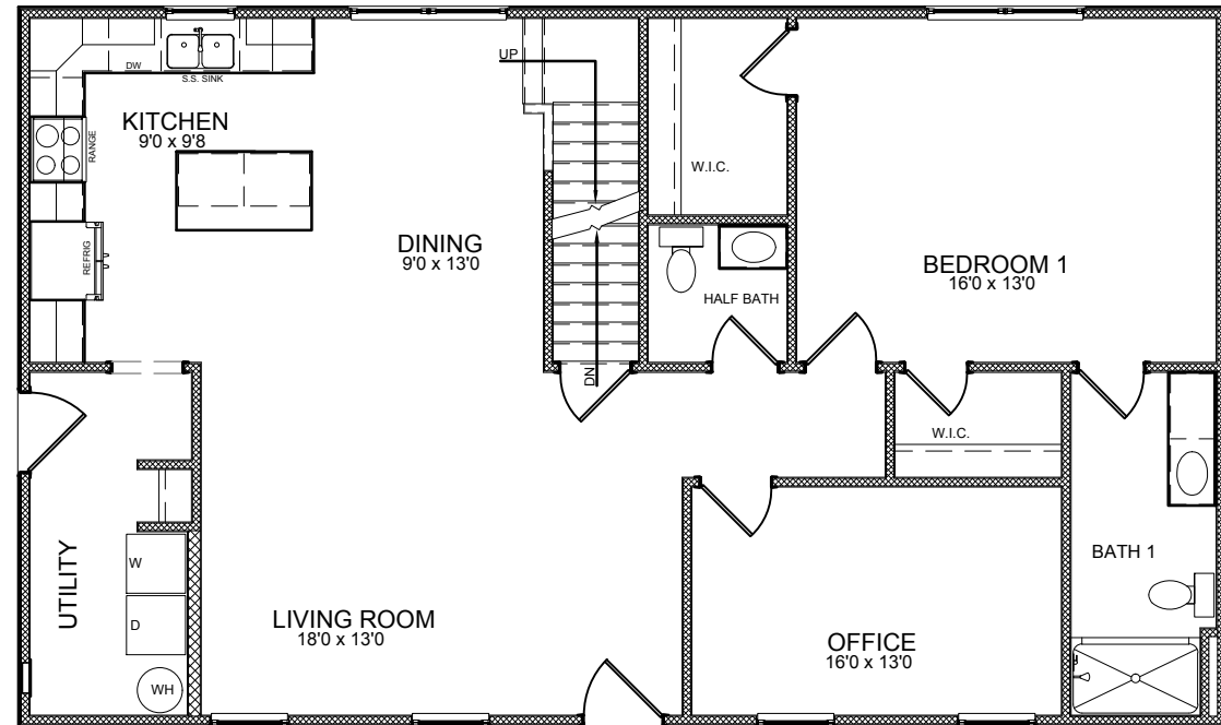
BASEMENT ACCESS OPTION
