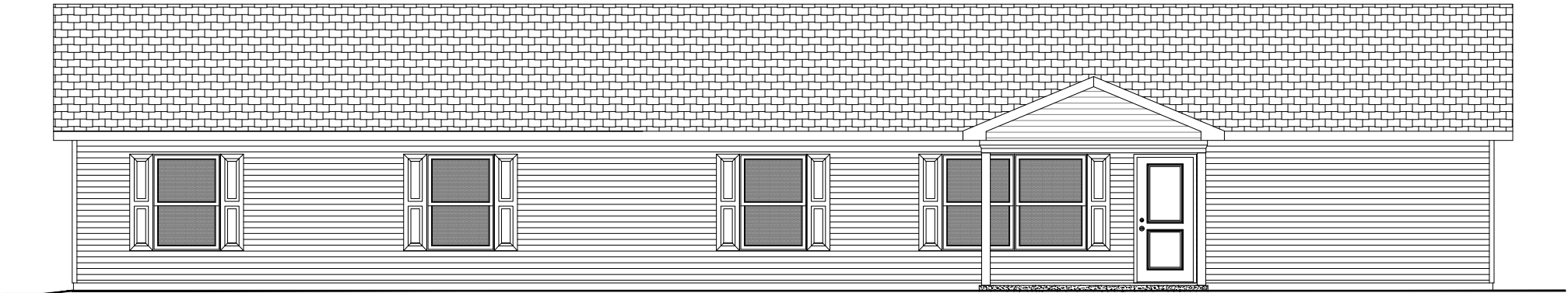
12' X 6' COVERED PORCH W/ GABLED ROOF
